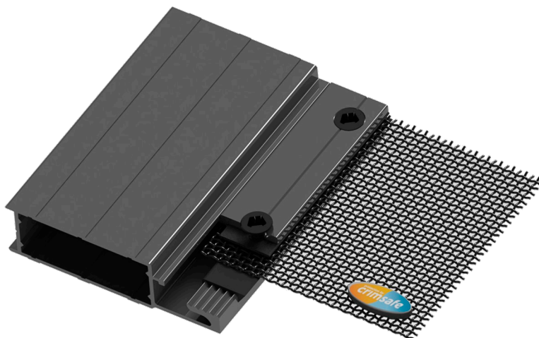
Cross section of mesh, frame and the screw clamp system.
