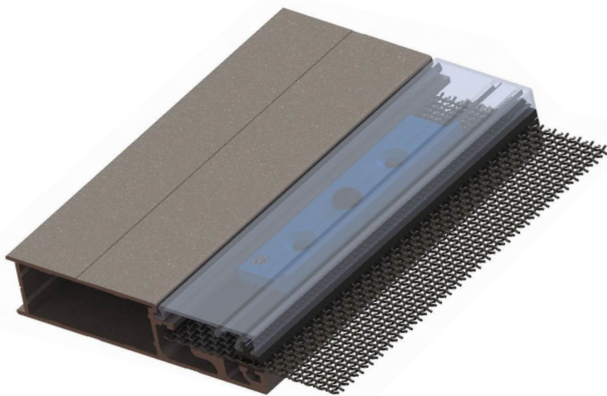
Cross section of mesh and frame featuring the New Carbon Fibre Screw-clamp 'clip' system.
